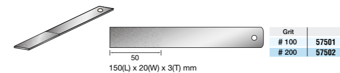
150(L) x 20(W) x 3(T) mm Grit # 100 57501 # 200 57502
